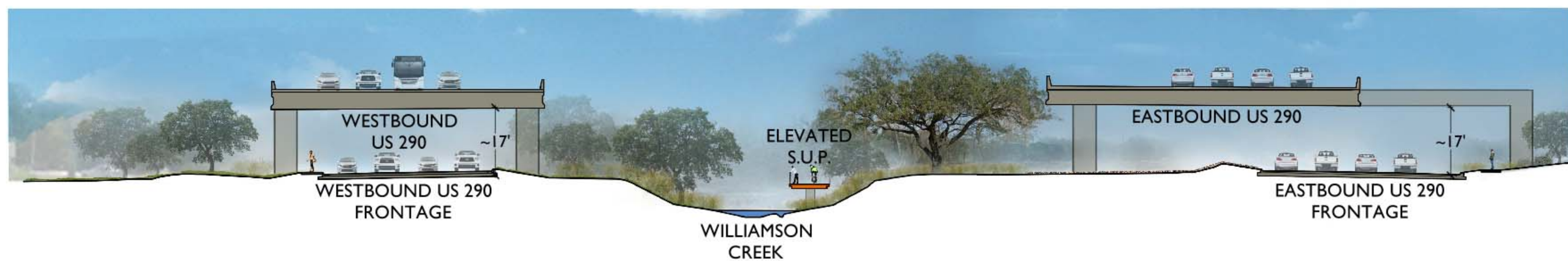
SECTION THROUGH WILLIAMSON CREEK NEAR WILLIAM CANNON DRIVE - ALTERNATE A
