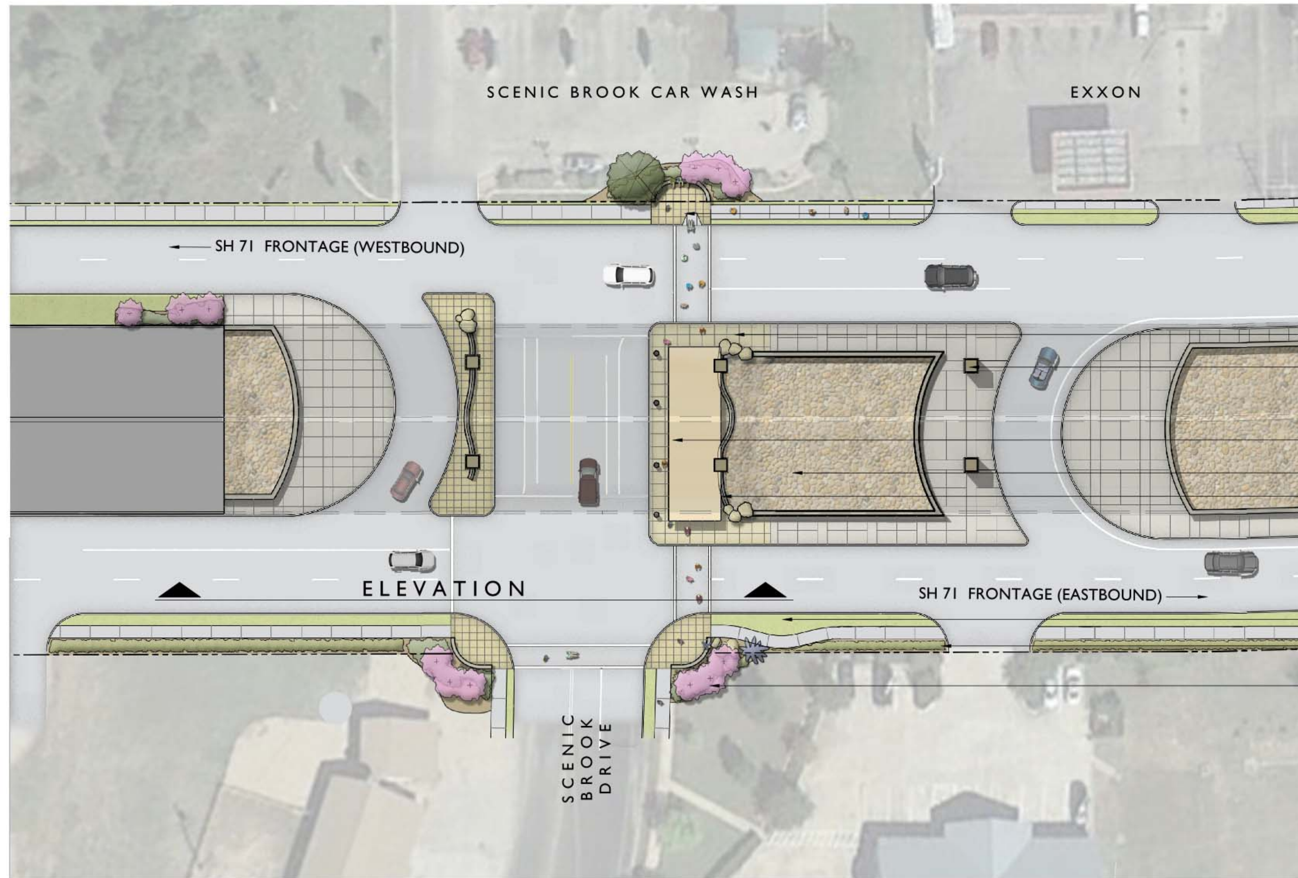
SCENIC BROOK DRIVE - PLAN VIEW
