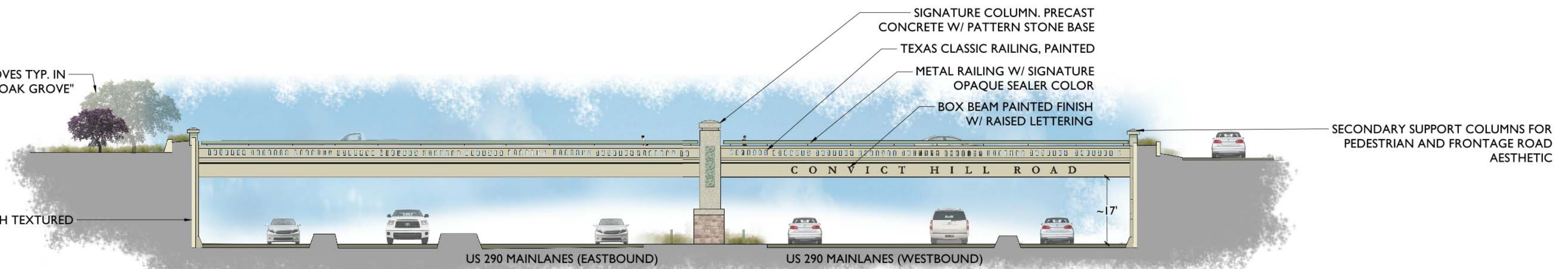
CONVICT HILL ROAD - SECTION VIEW
