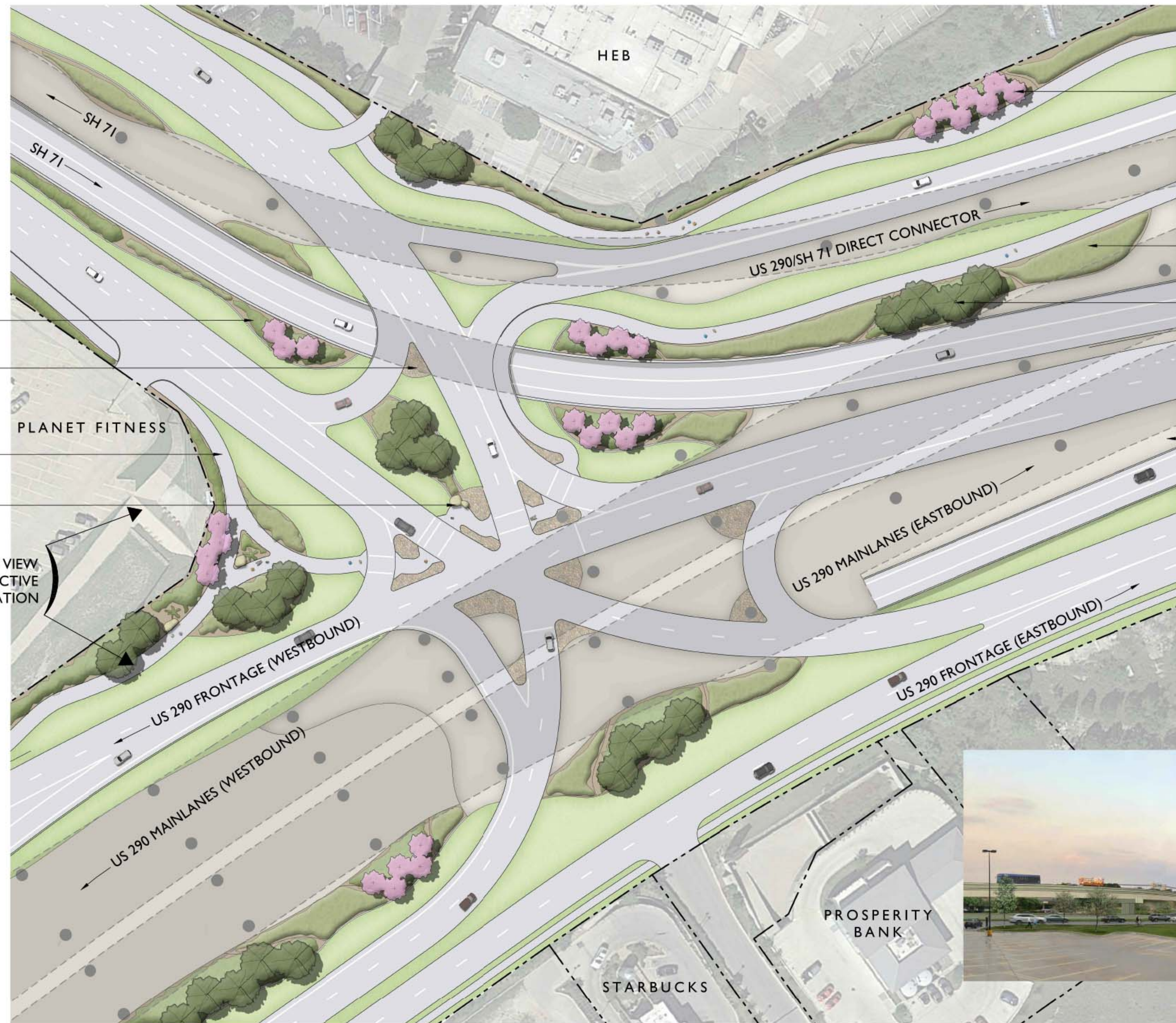
US 290/HWY 71 INTERCHANGE - PLAN VIEW - ALTERNATE C
