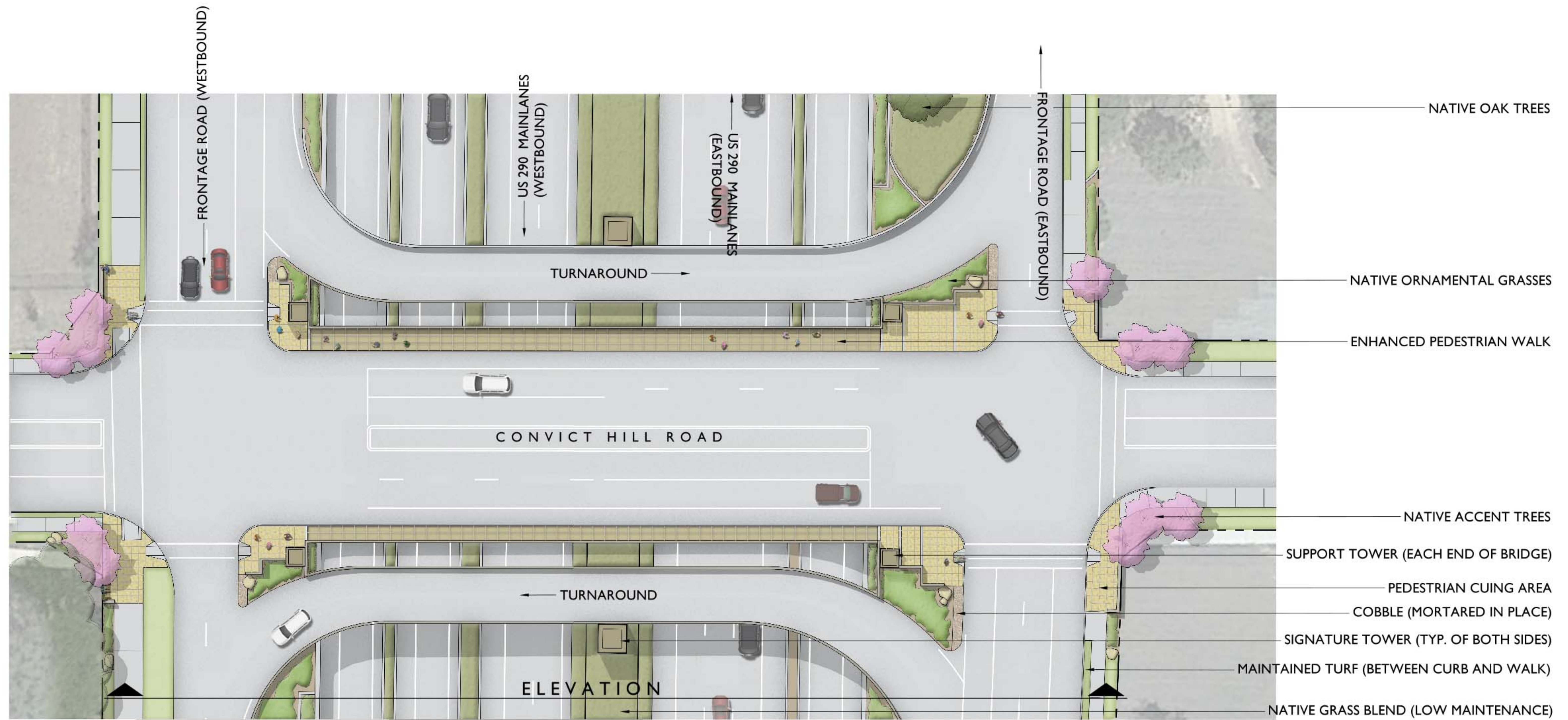
CONVICT HILL ROAD - PLAN VIEW
