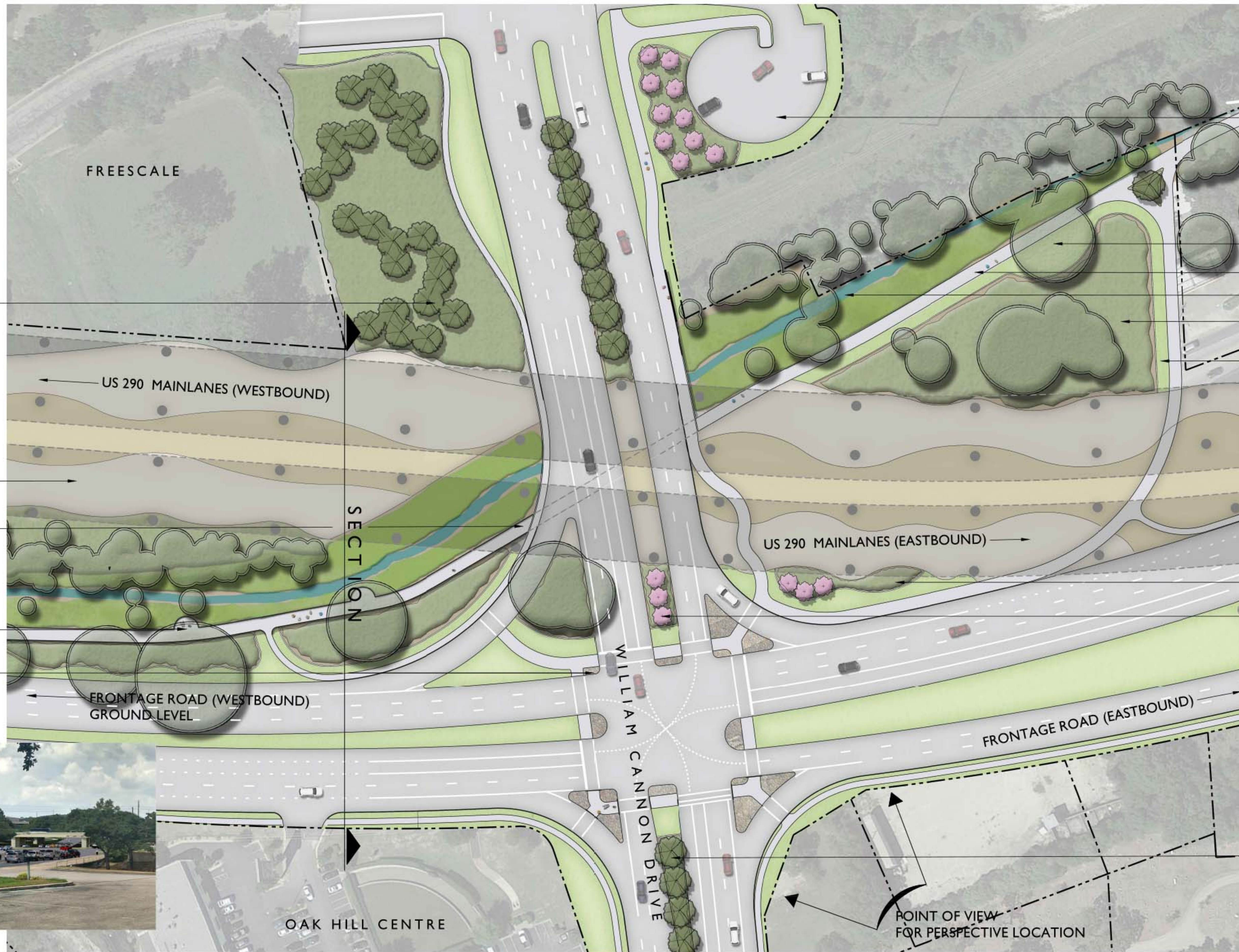
WILLIAM CANNON DRIVE - PLAN VIEW - ALTERNATE C
