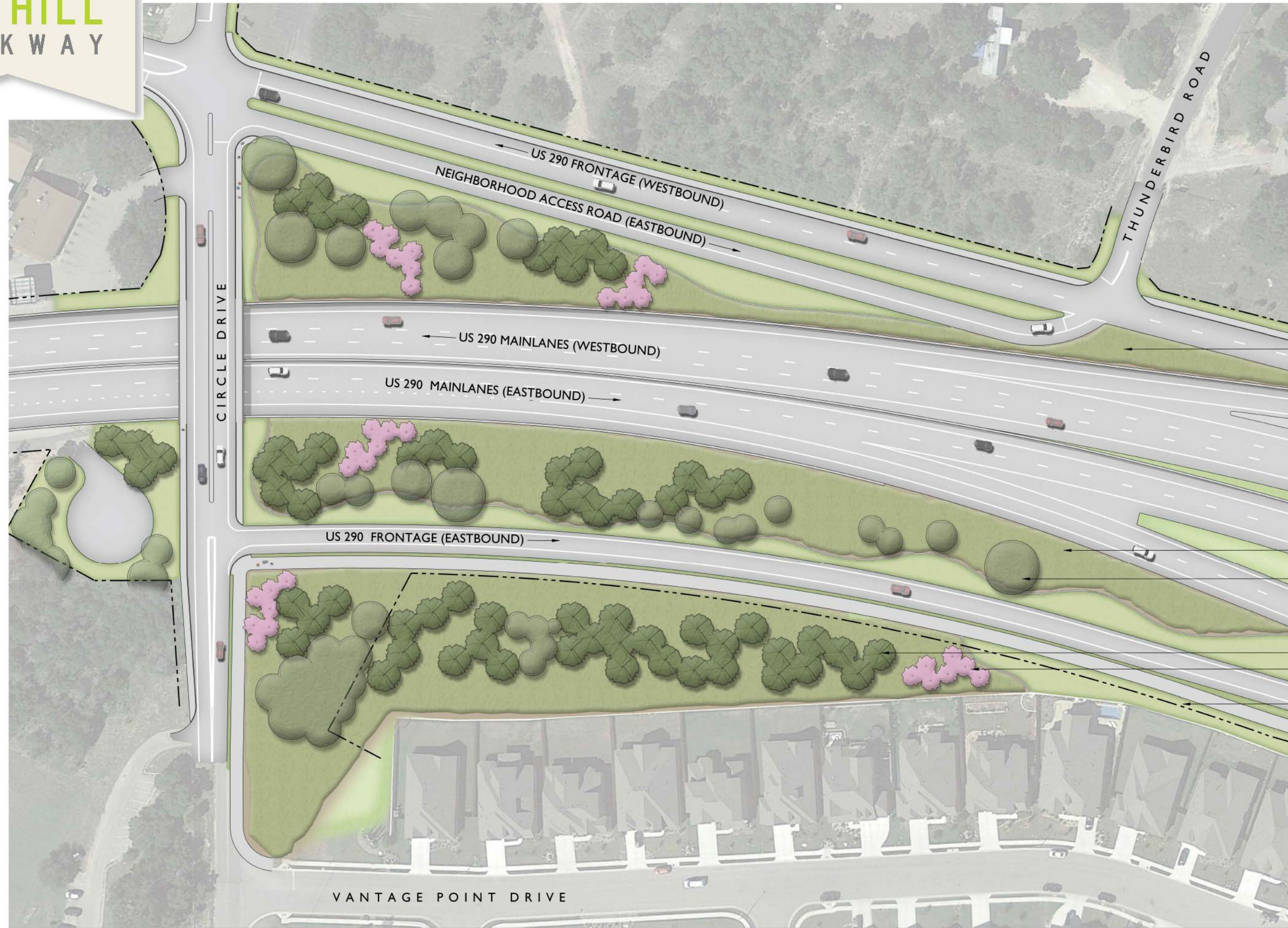
CIRCLE DRIVE - PLAN VIEW
