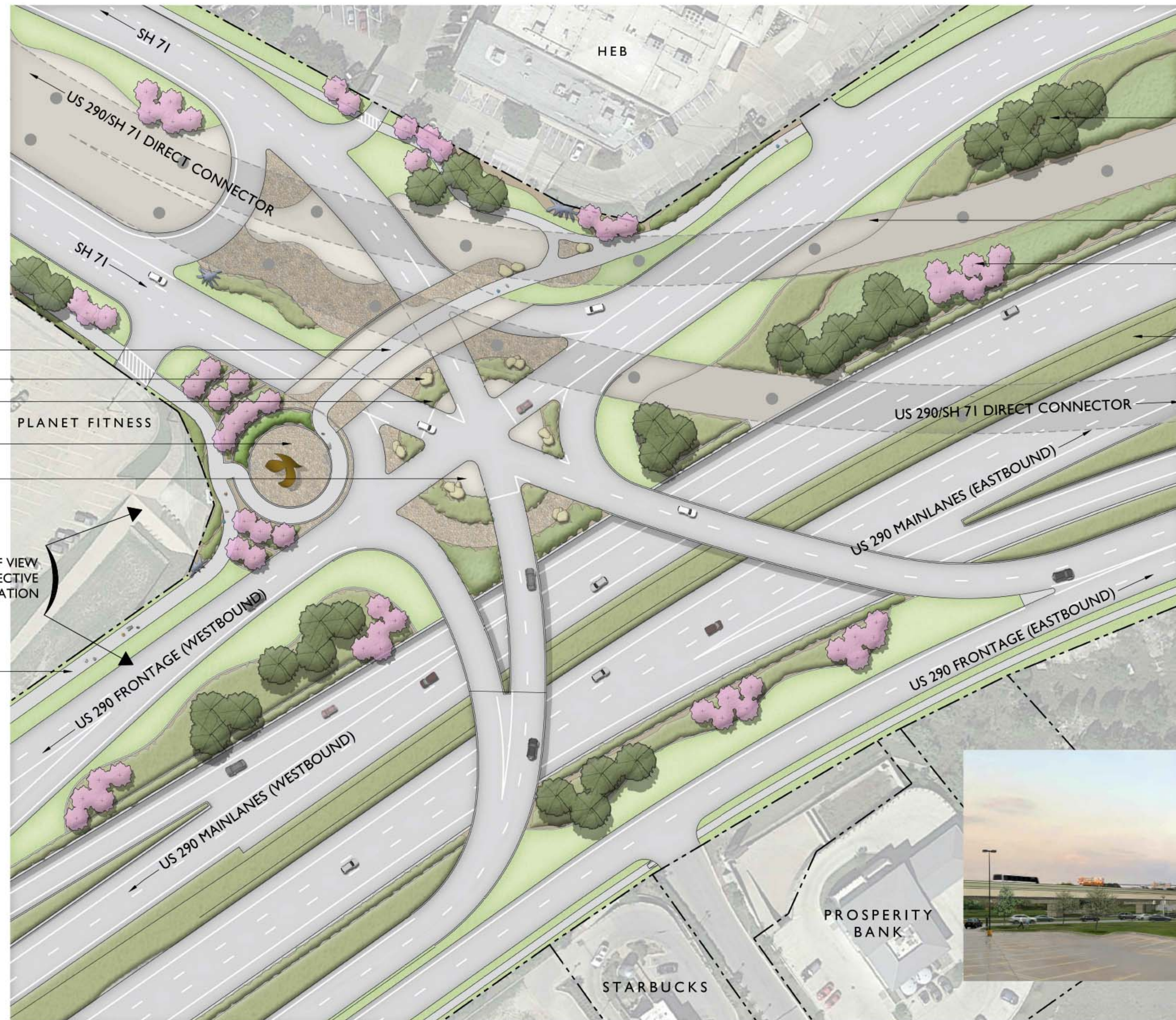
US 290/HWY 71 INTERCHANGE - PLAN VIEW - ALTERNATE A
